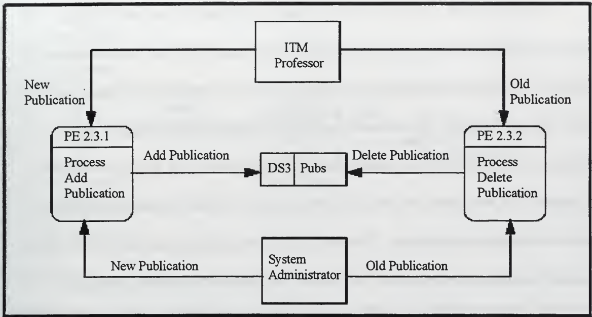
Figure 9. Primitive Level DFD For Maintaining Publications
